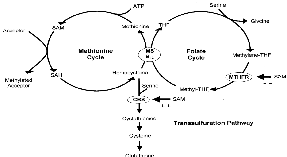
Fig. 1. One-carbon metabolism.
